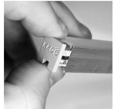
For surface wiring replace solid end cap/s with notched end cap/s supplied.
